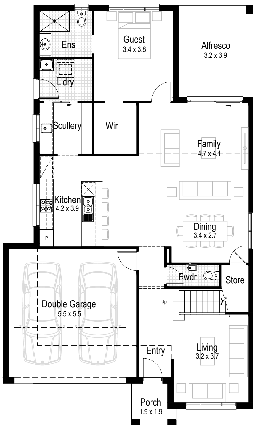
Ground Floor
